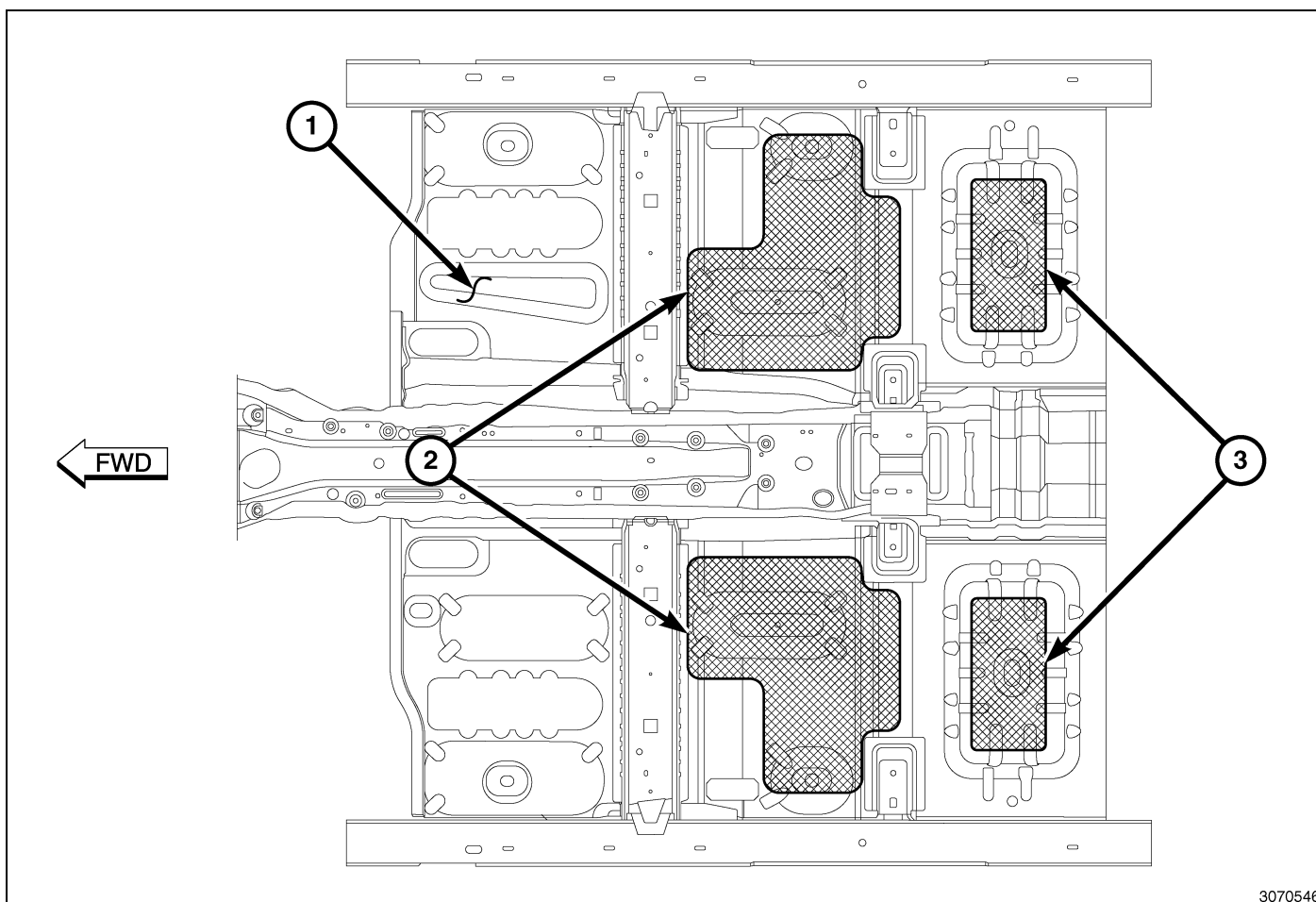
Fig. 24 Mid Floor Pan
