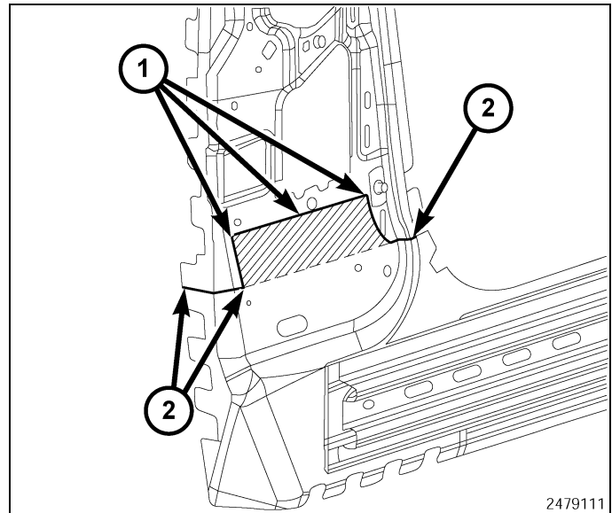
Fig. 12 Modified Lap Joint
