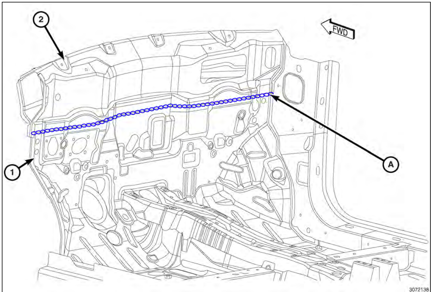
Fig. 29 Dash to Cowl
