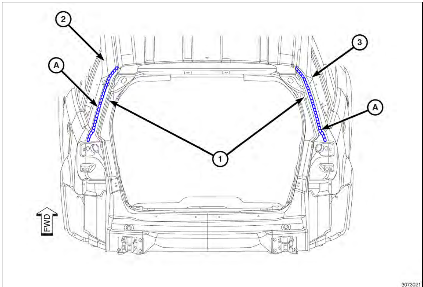
Fig. 53 Body Side Aperture To Drain Trough
