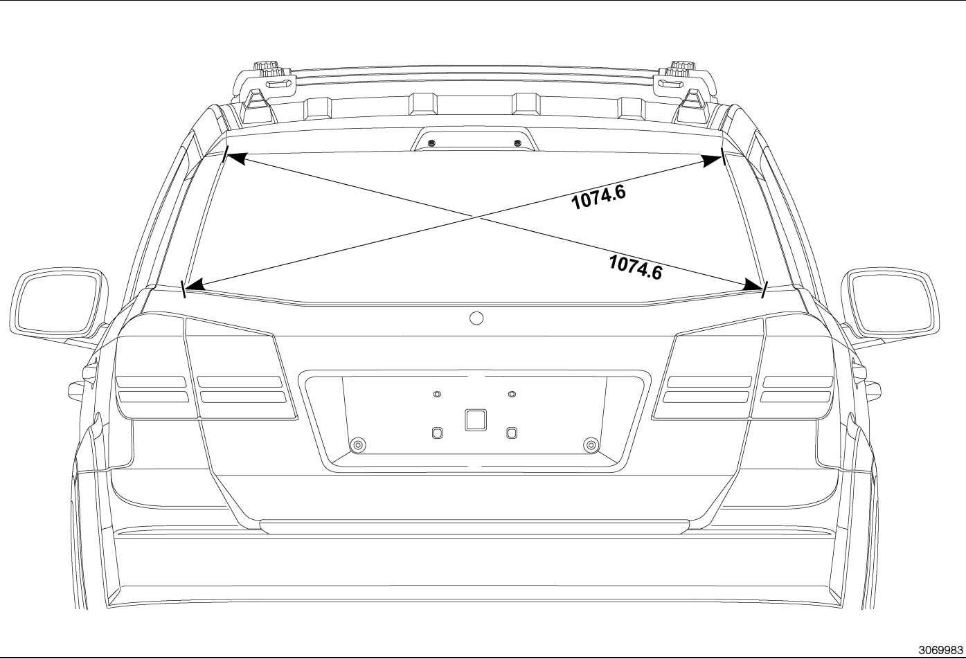
Fig. 6 Liftgate Glass
