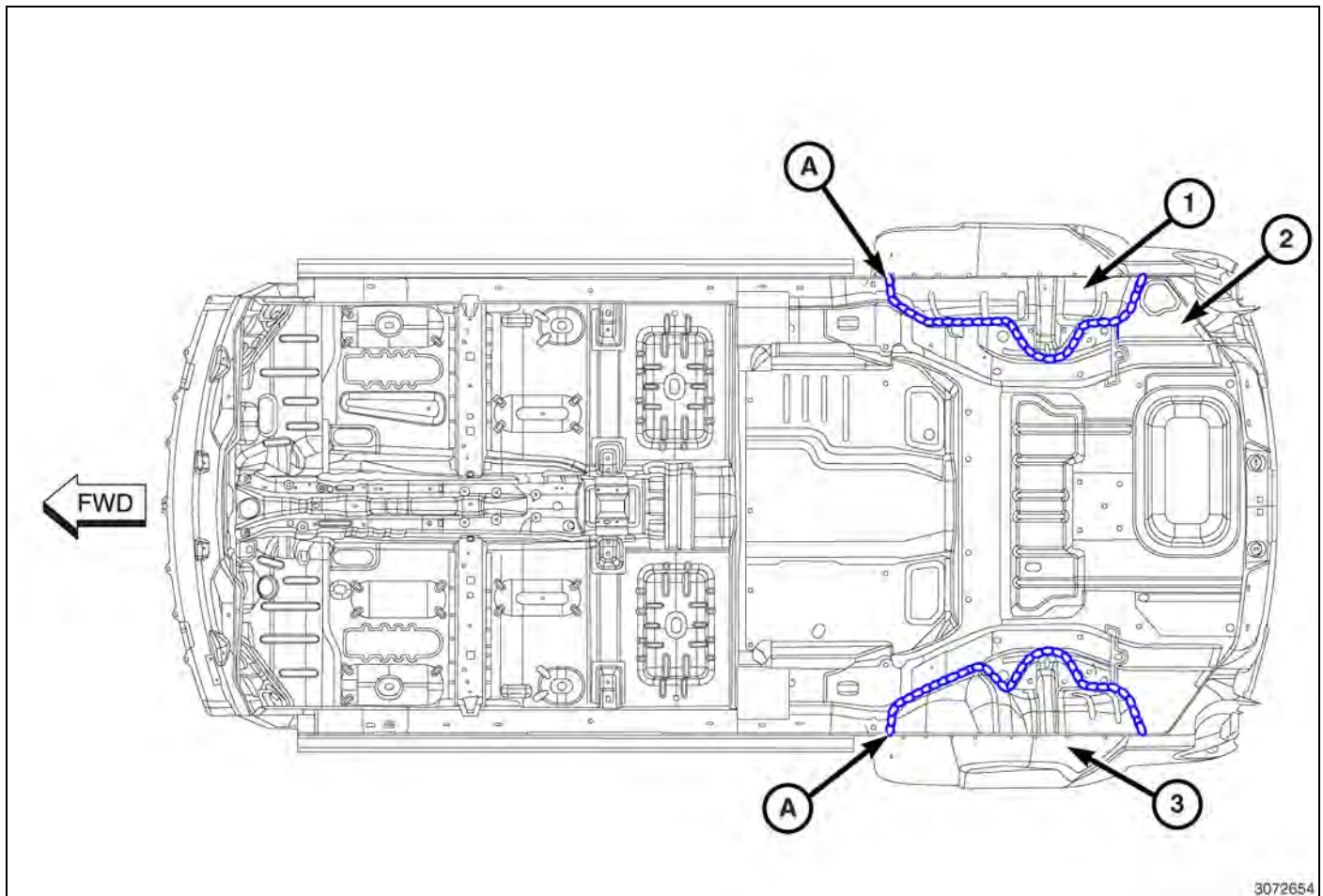
Fig. 44 Rear Wheelhouse To Rear Floor Pan
