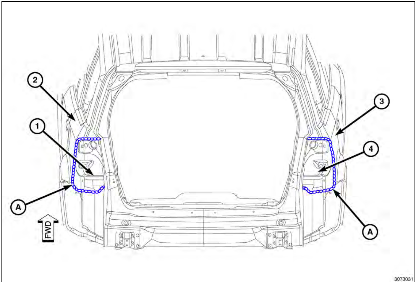
Fig. 54 Body Side Aperture To Tail Lamp Housing Panel
