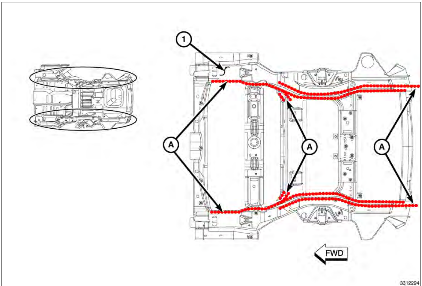
Fig. 69 Rear Floor
