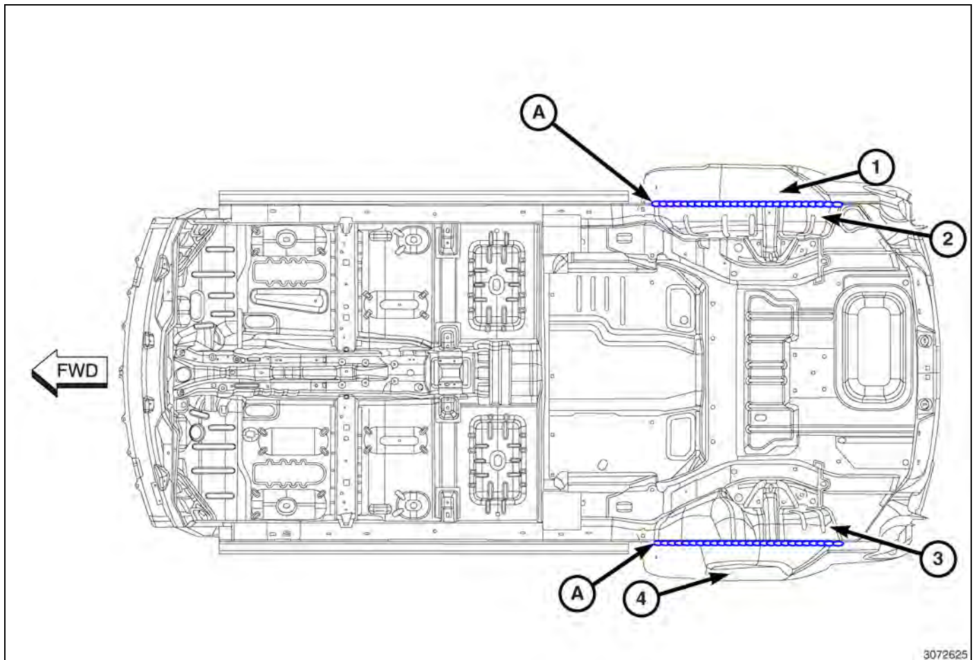
Fig. 42 Rear Wheelhouse To Inner Body Side Aperture
