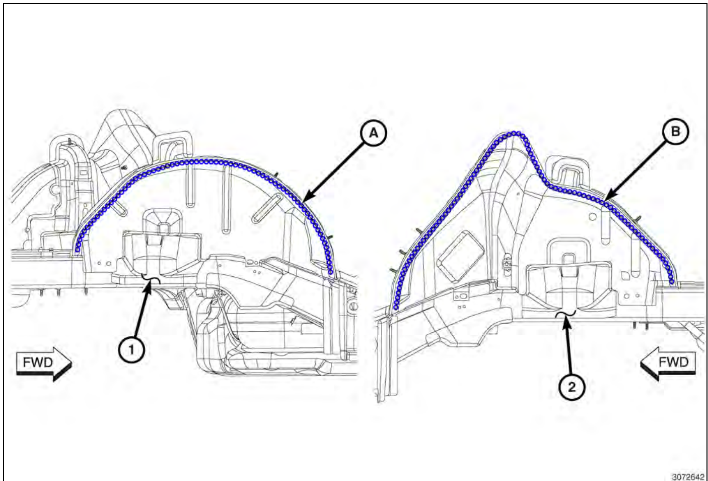
Fig. 43 Inner Wheelhouse To Inner Body Side Aperture
