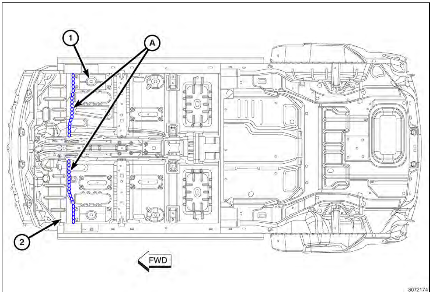
Fig. 33 Front Floor Pan To Dash
