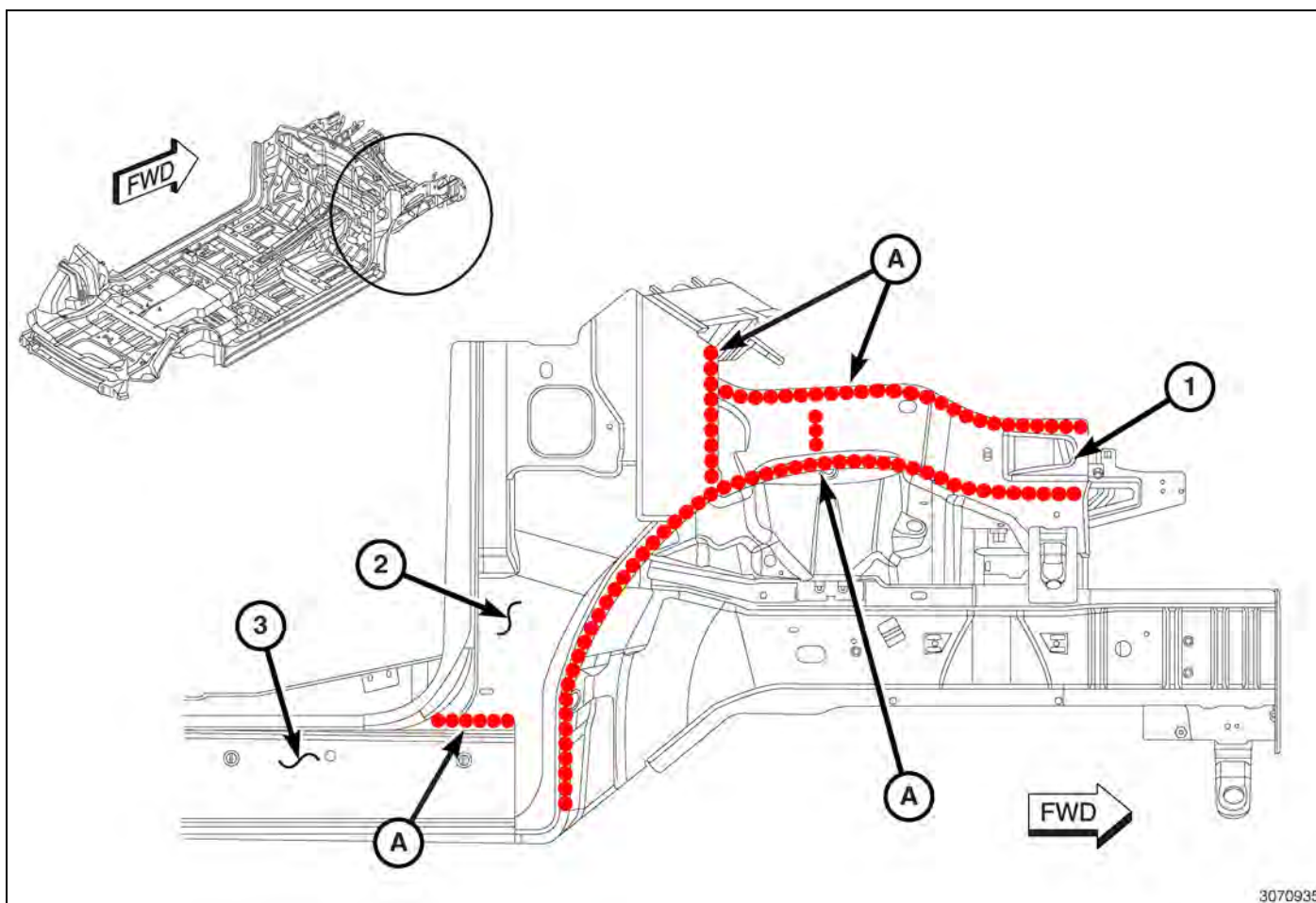
Fig. 58 Cowl Side/Engine Box
