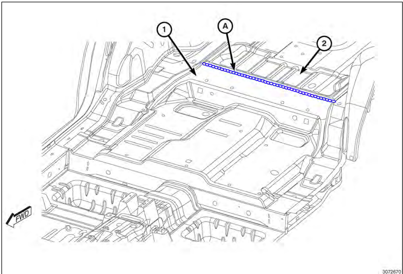
Fig. 45 Third Row Crossmember To Rear Floor Pan
