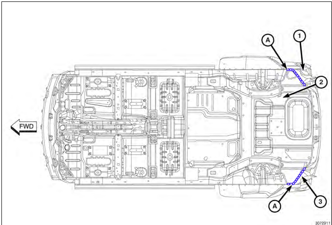
Fig. 48 Rear Floor Pan To Inner Body Side Aperture
