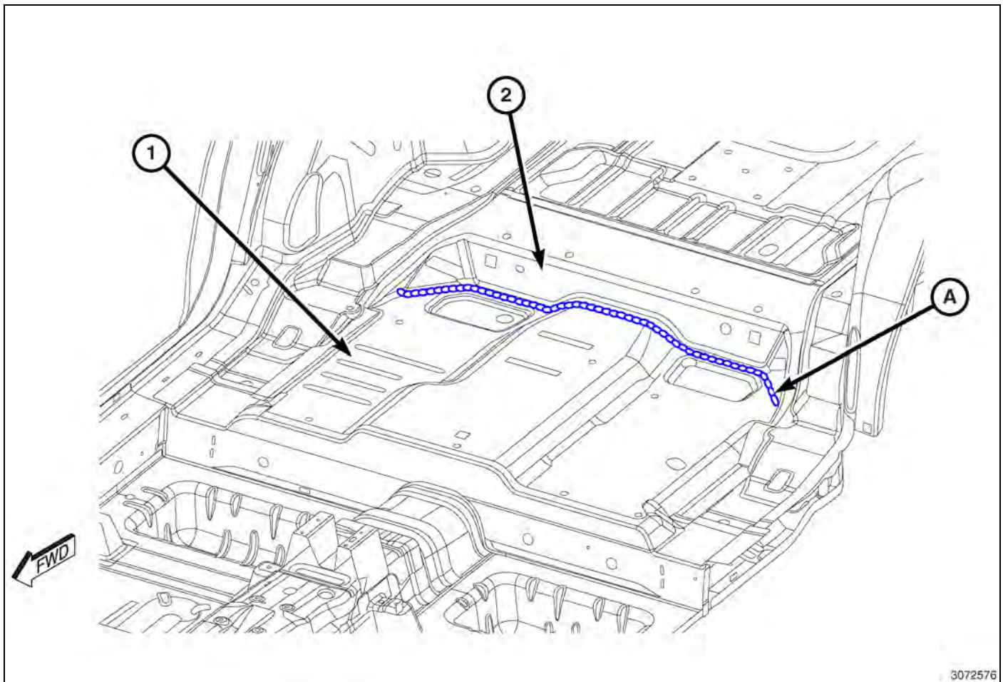
Fig. 40 Mid Floor Pan To Third Row Crossmember
