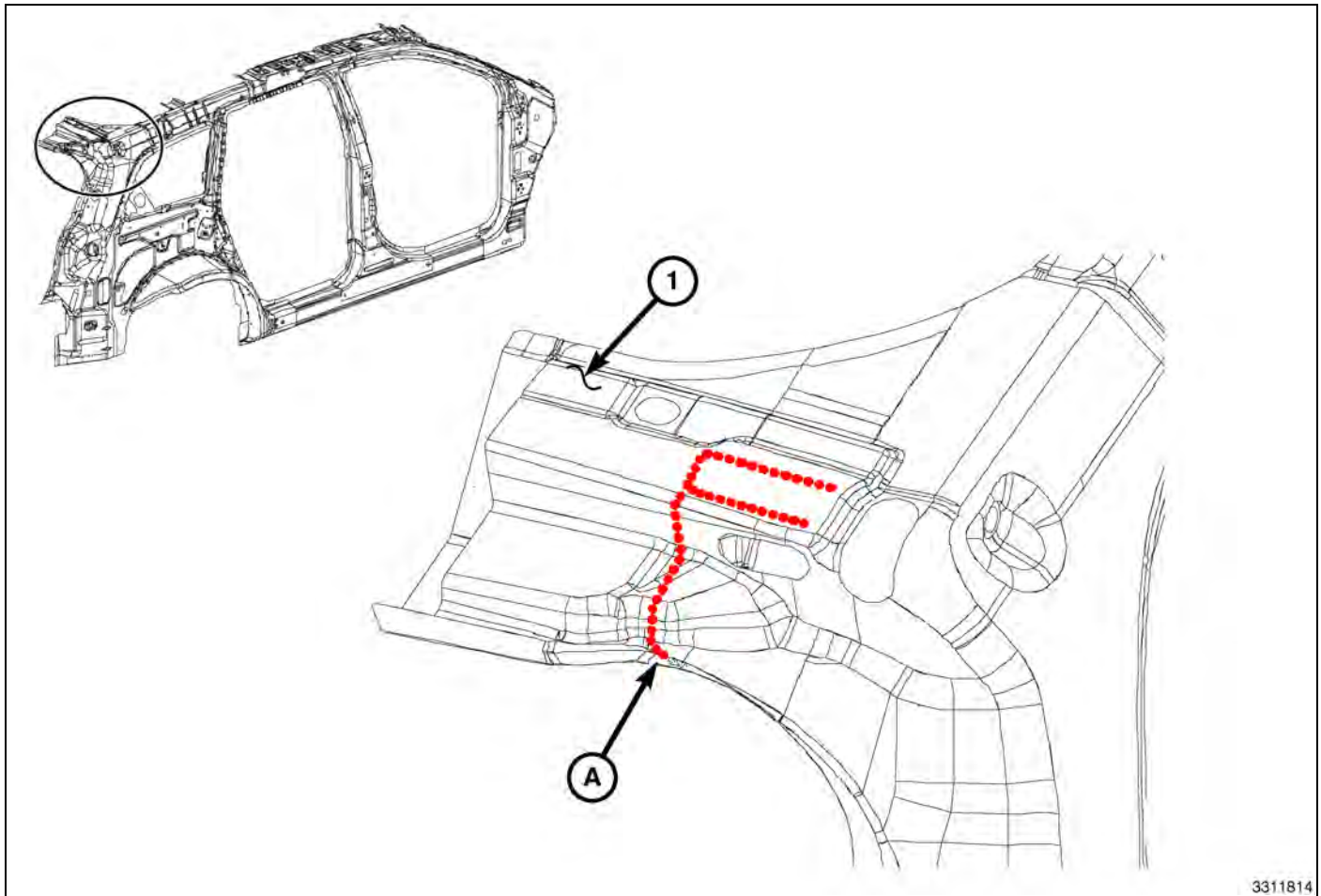
Fig. 76 D-PILLAR
