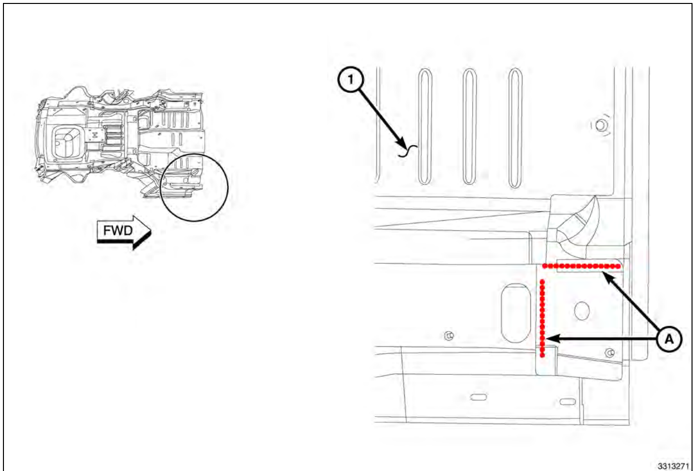
Fig. 67 Mid Floor
