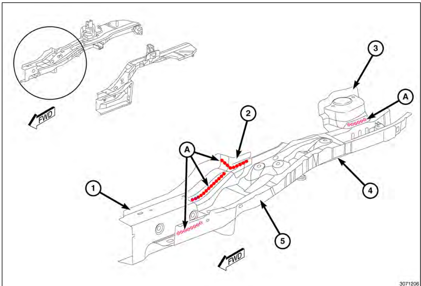
Fig. 64 Side Member (1 of 2)
