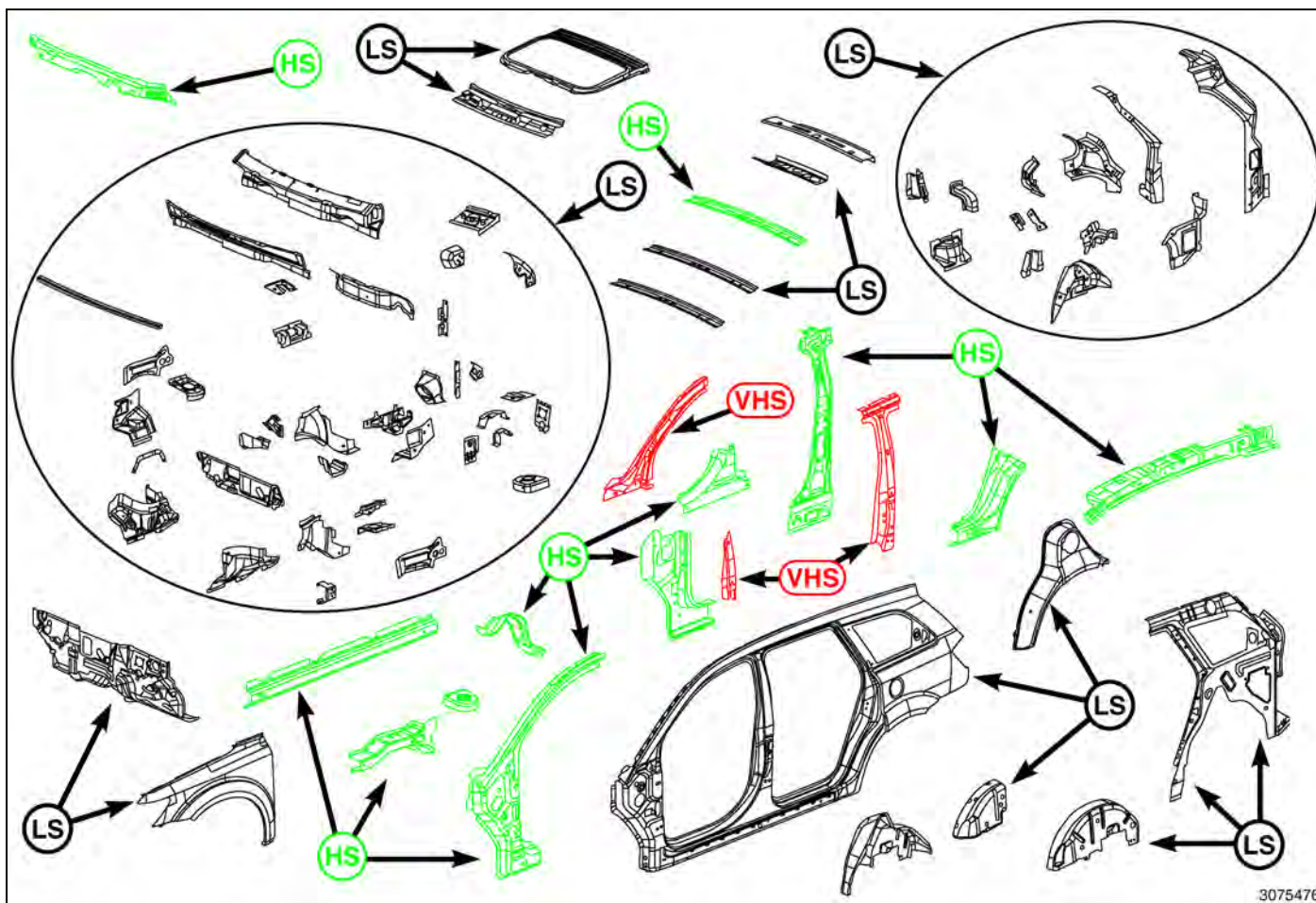
Body In White Components - Upper Structure
