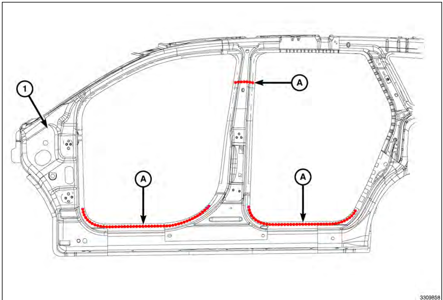
Fig. 62 Inner Body Side aperture
