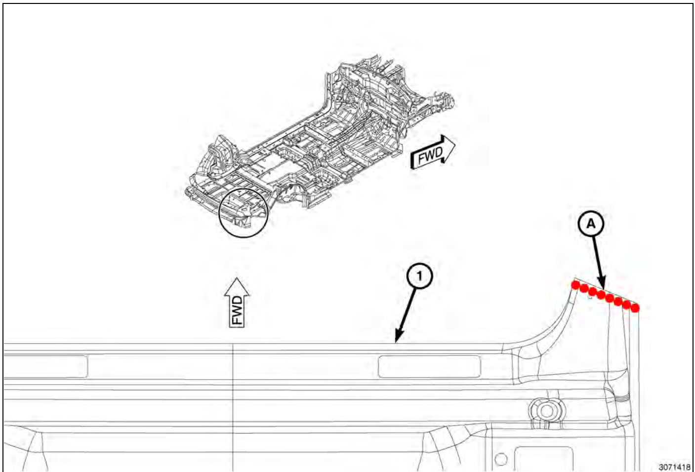
Fig. 75 Lower Liftgate Opening Crossmember
