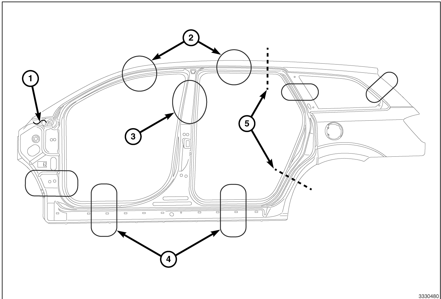
Fig. 20 Outer Body Side Aperture
