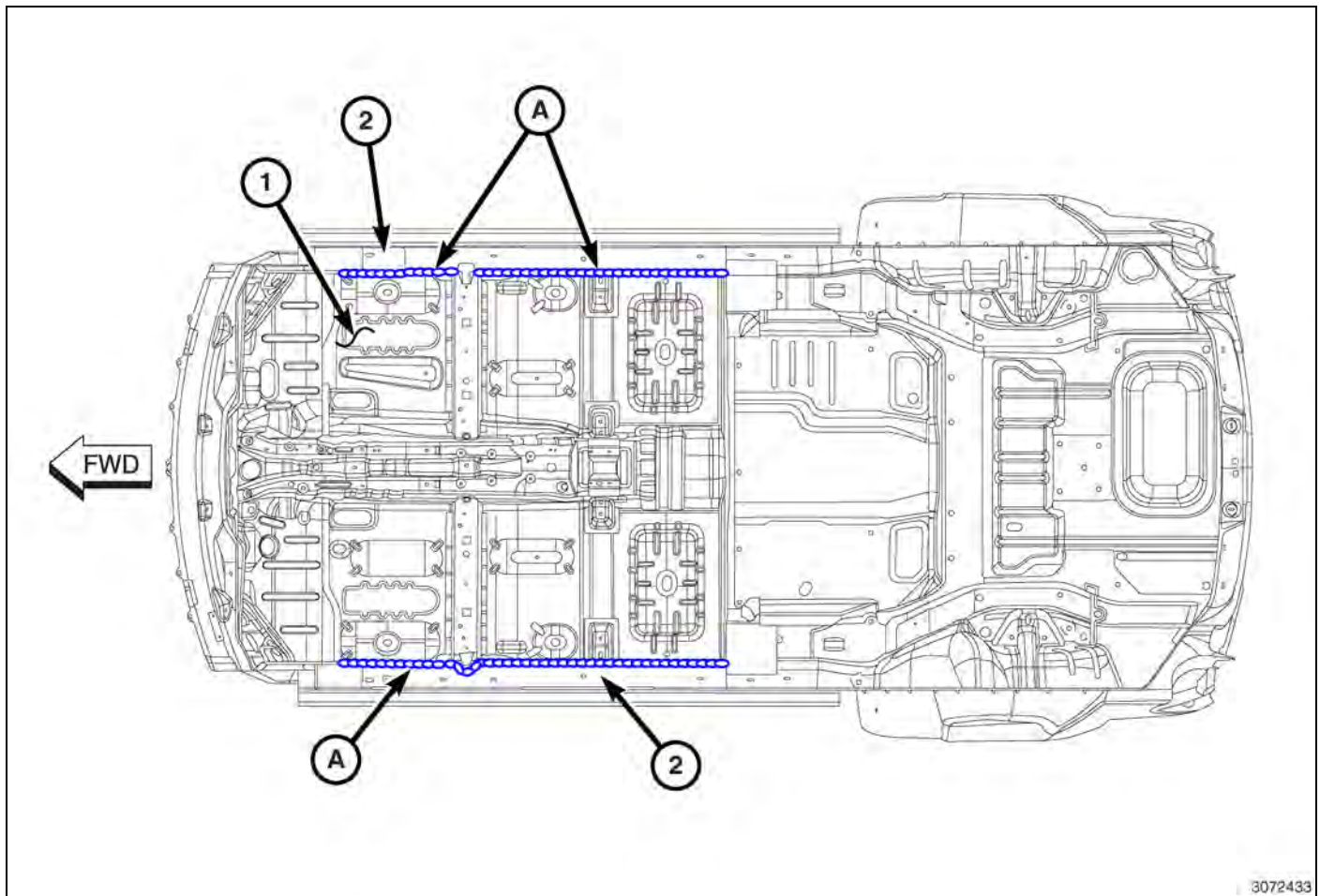
Fig. 34 Front Floor Pan To Sill
