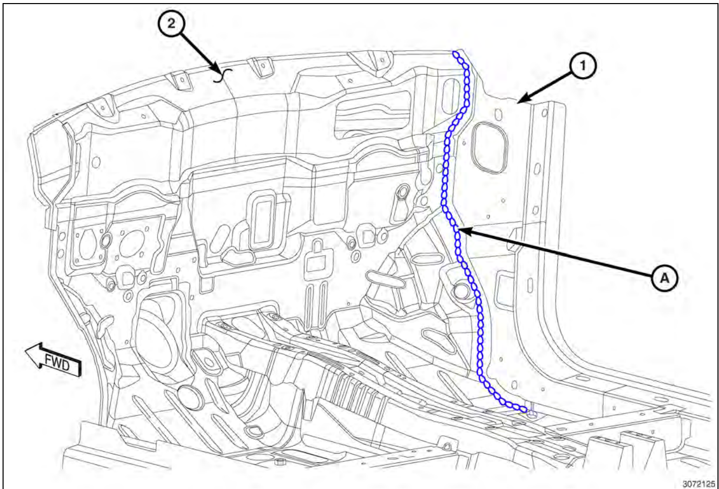
Fig. 28 Cowl Side to Dash/Cowl
