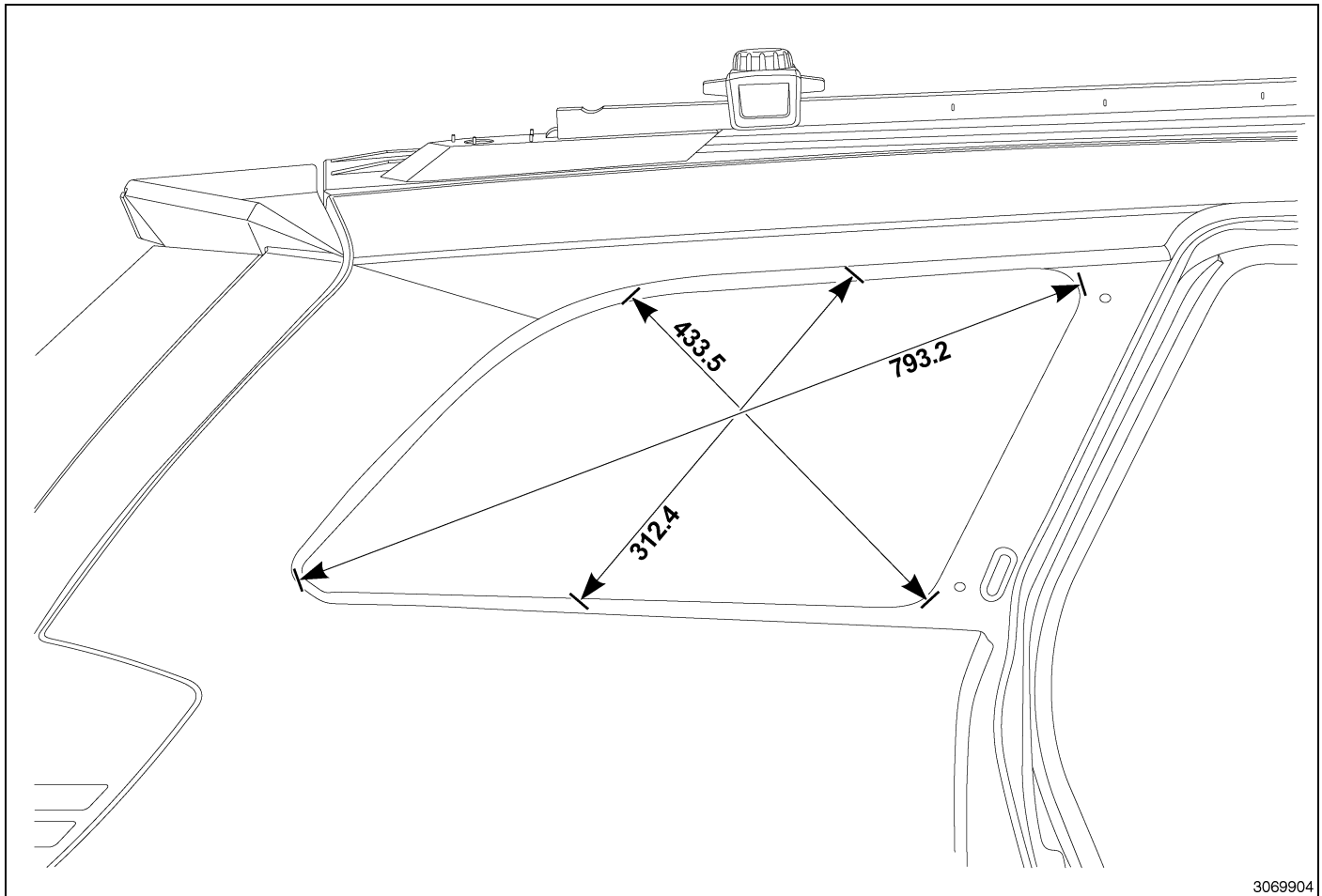
Fig. 4 Quarter Glass
