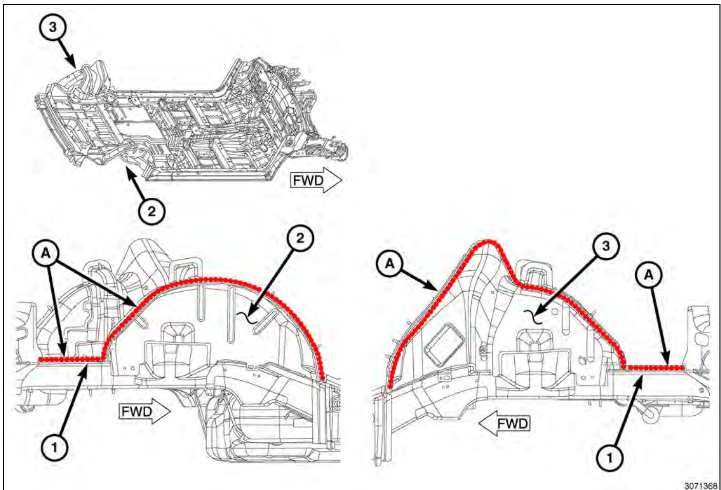
Fig. 70 Rear Floor/Body Side Aperture
