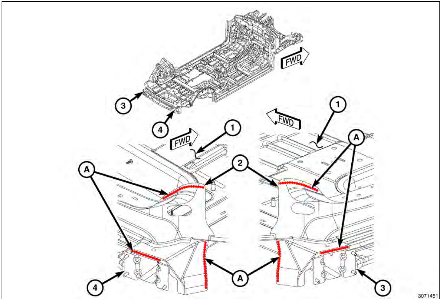
Fig. 73 Rear Floor/Lower Liftgate Opening Crossmember
