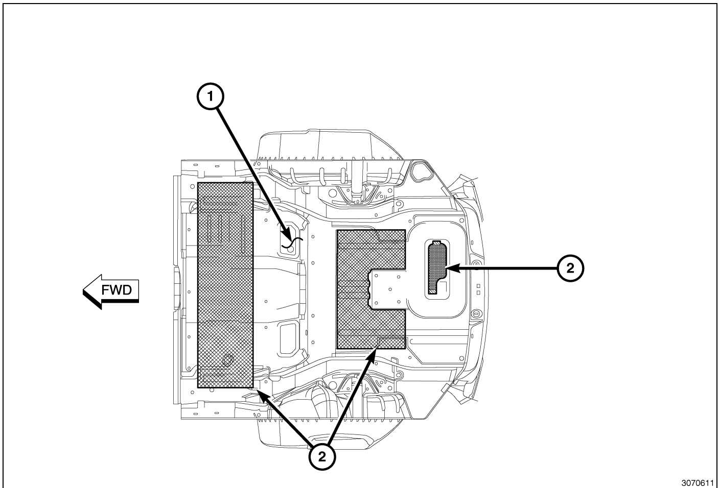
Fig. 25 Center/Rear Floor Pan
