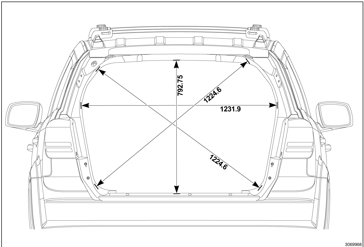
Fig. 5 Liftgate
