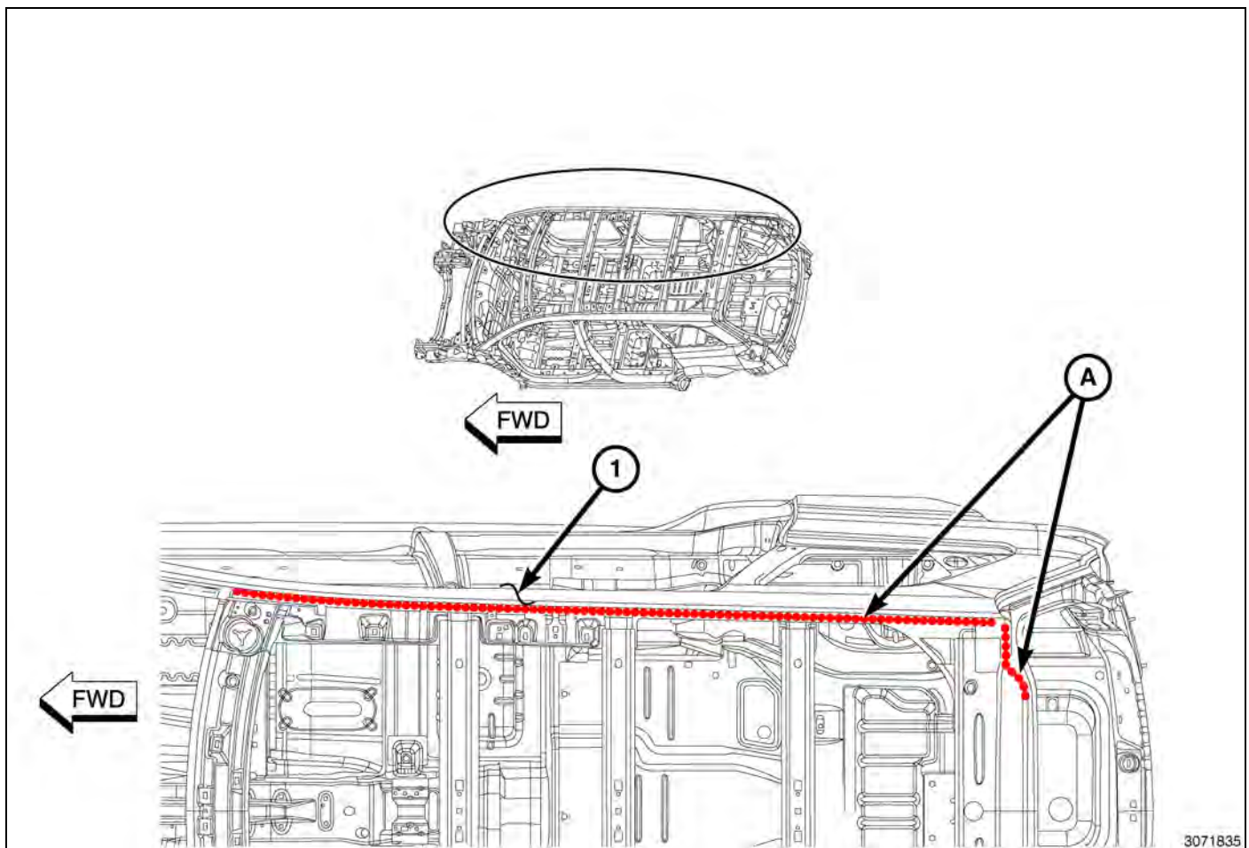
Fig. 80 Body Side Aperture/Roof Panel
