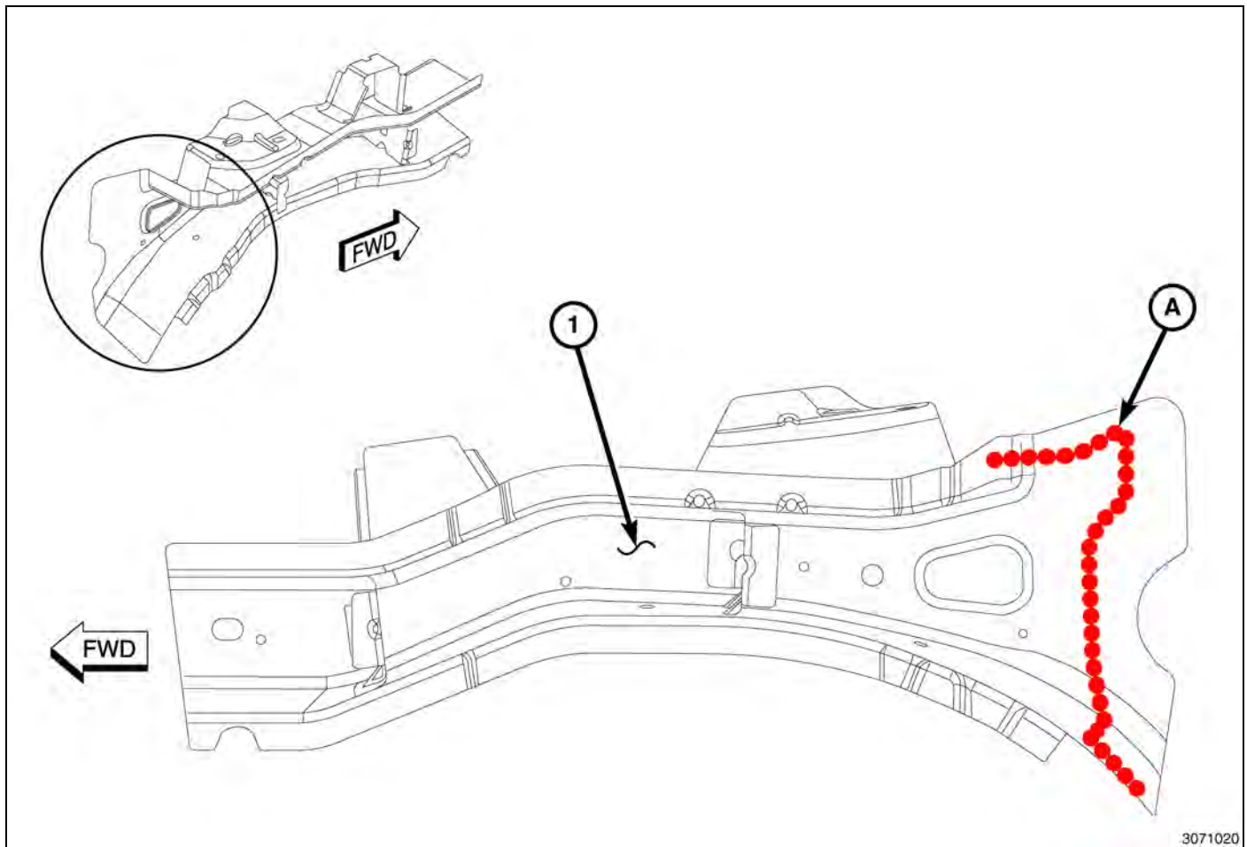
Fig. 59 Load Beam
