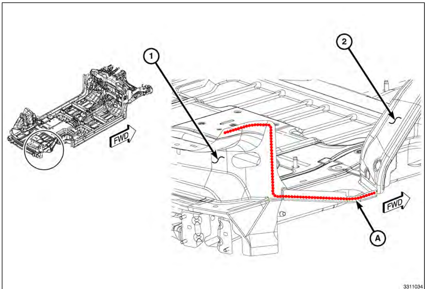
Fig. 74 Crossmember/Floor Extension
