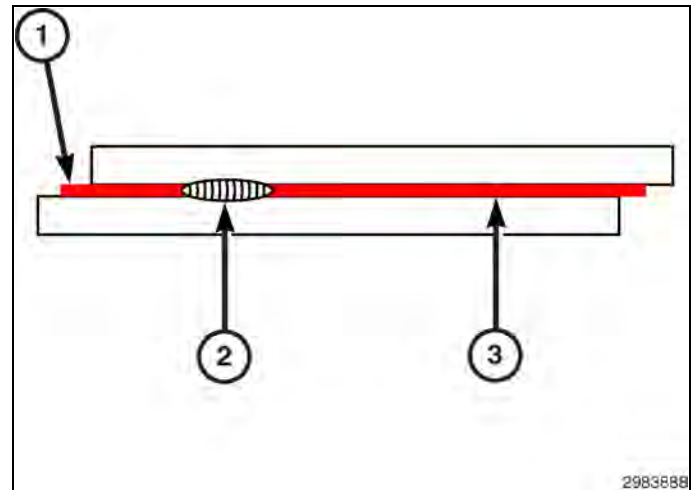
Fig. 14 Current Level Low for Both Welds
