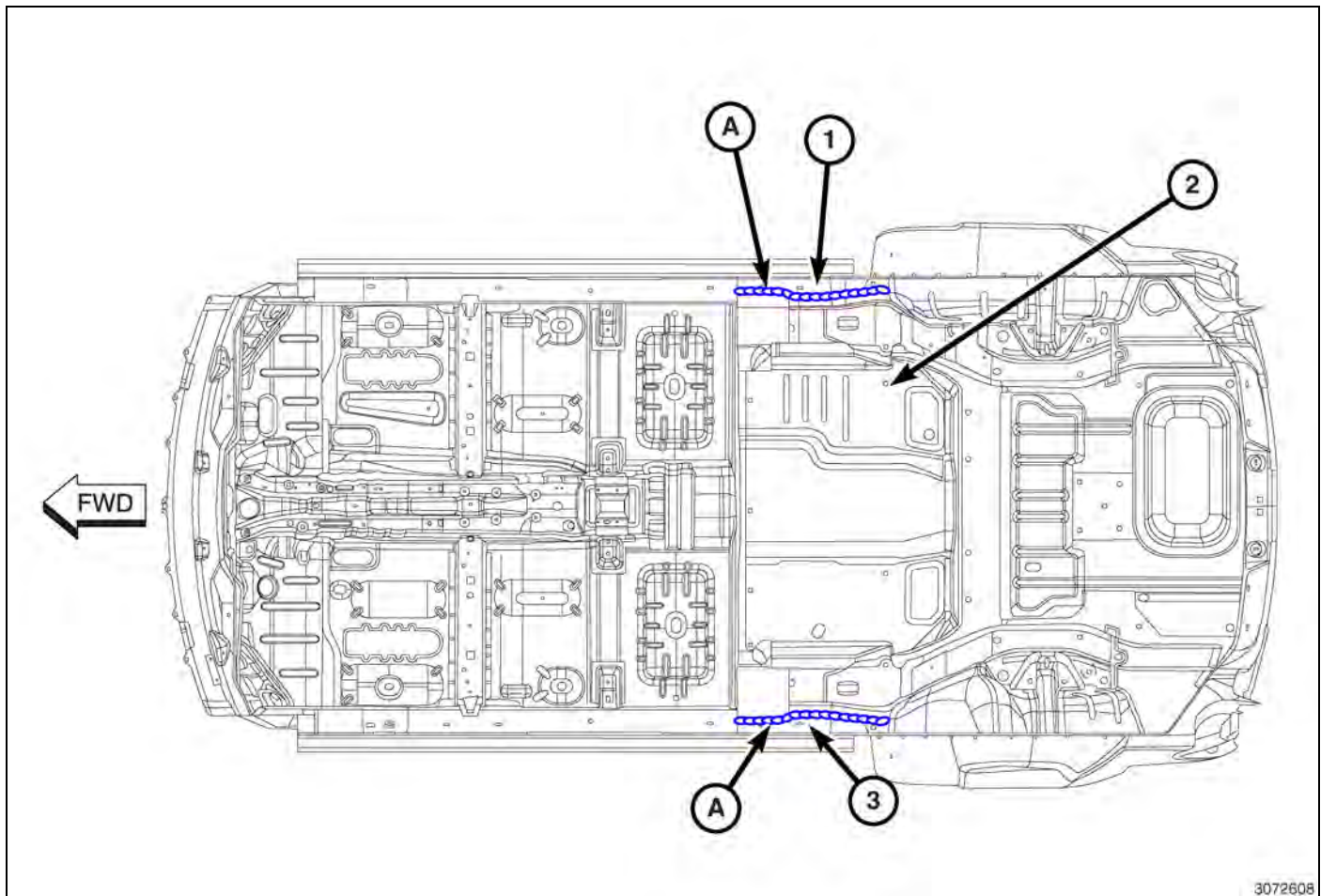
Fig. 41 Rear Sill To Rear Floor Pan
