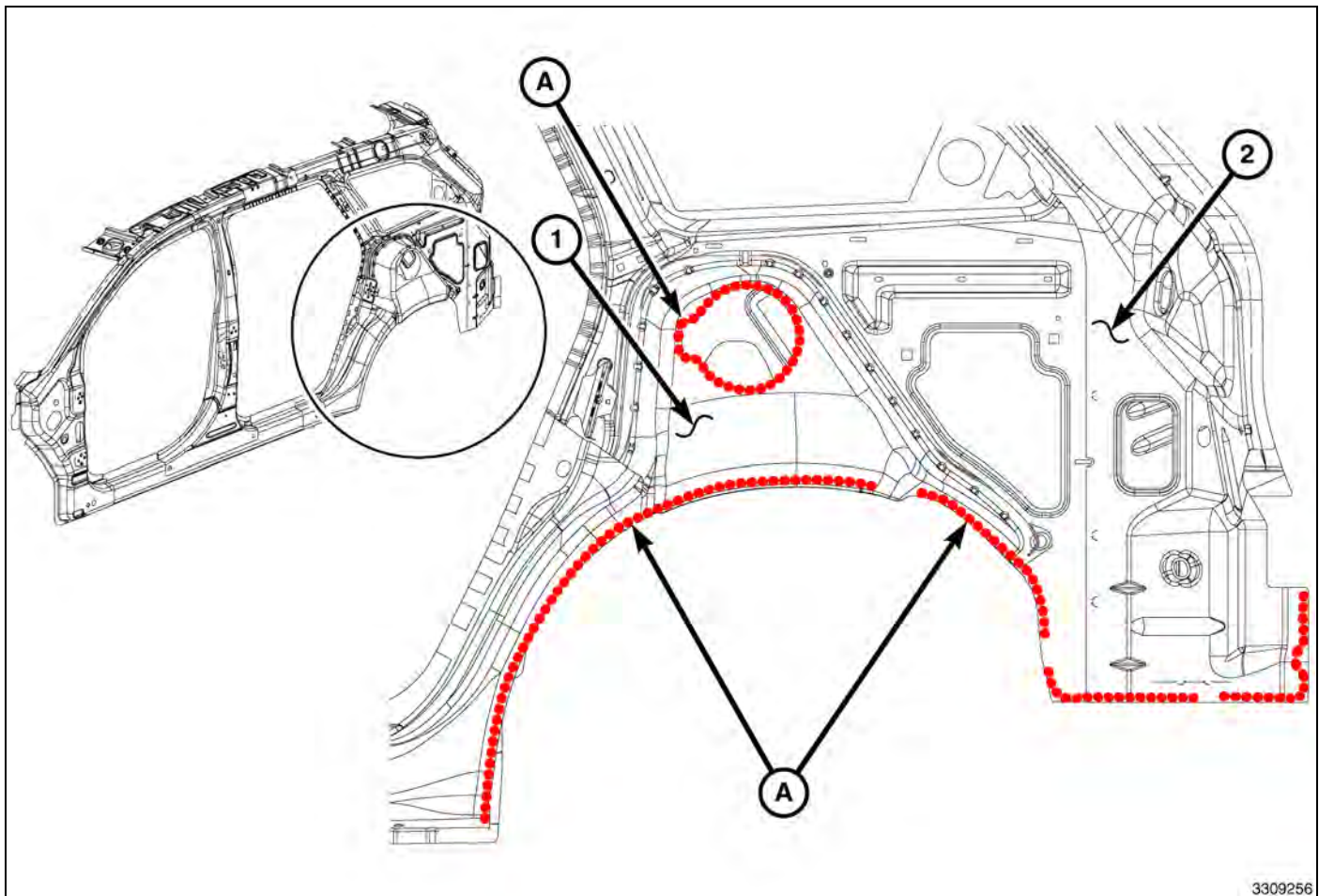
Fig. 72 Left Outer Wheelhouse
