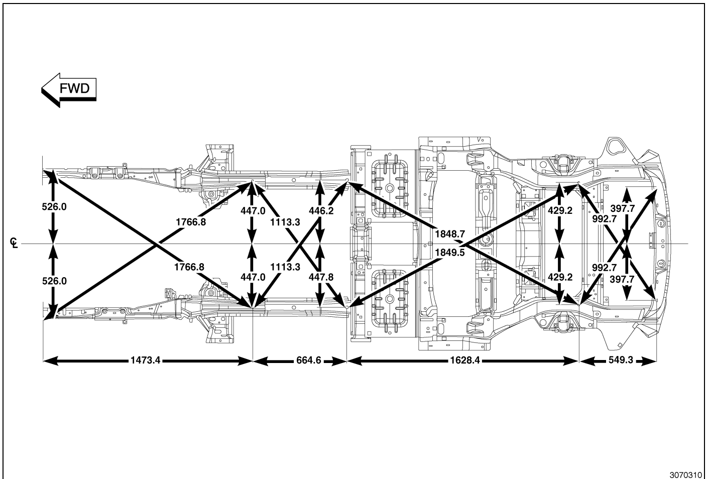
Fig. 7 Underbody Bottom View
