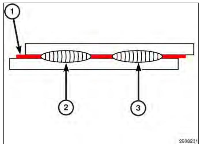
Fig. 19 Current Level Medium (2) High (3)
