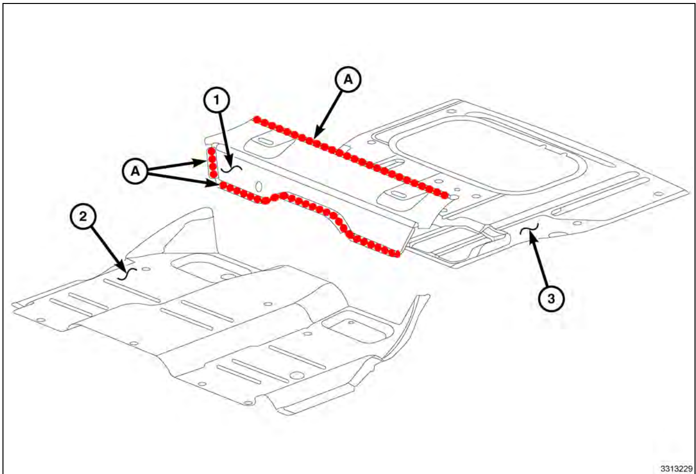
Fig. 68 3rd Row Seat Crossmember
