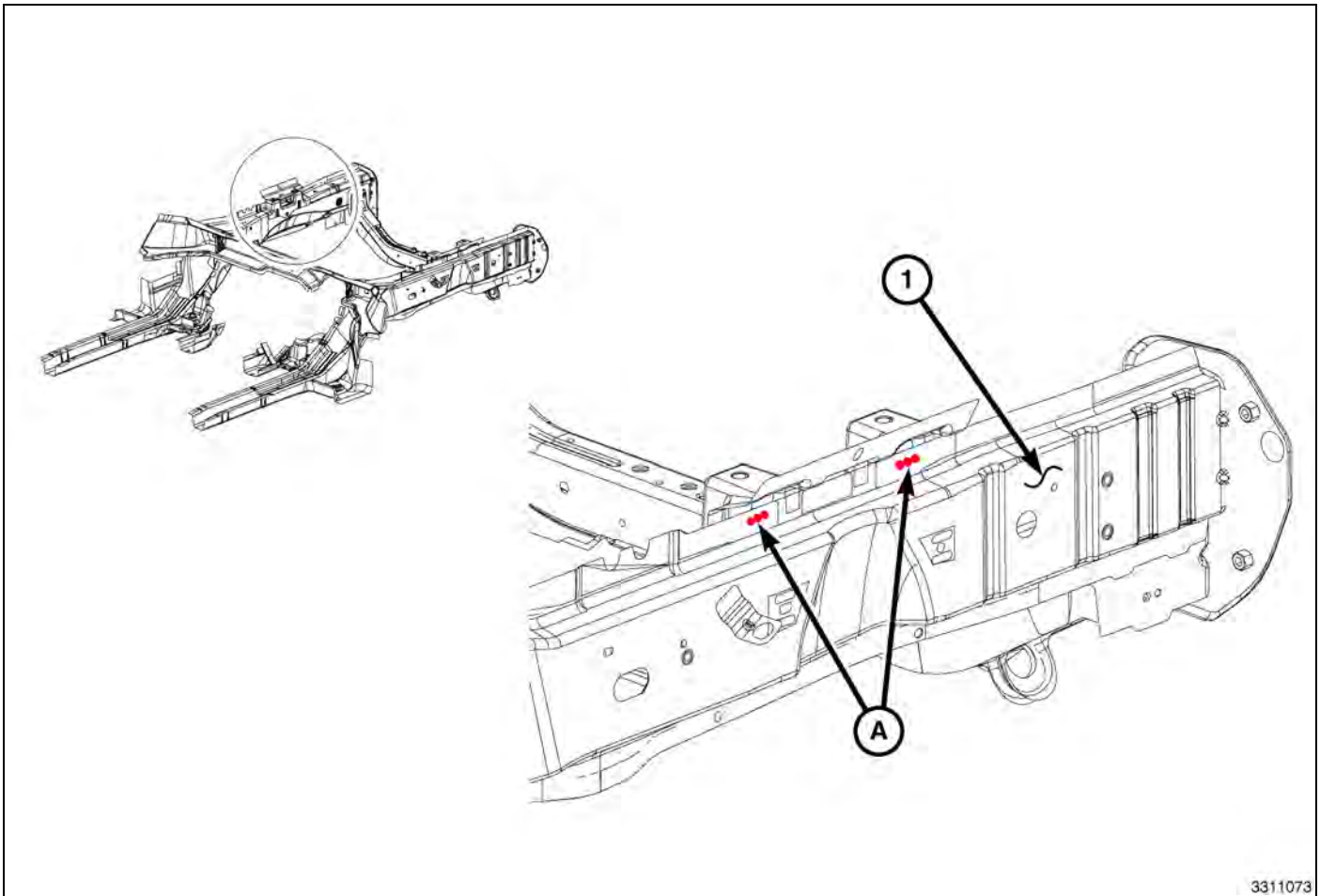
Fig. 57 Front Rail Lower
