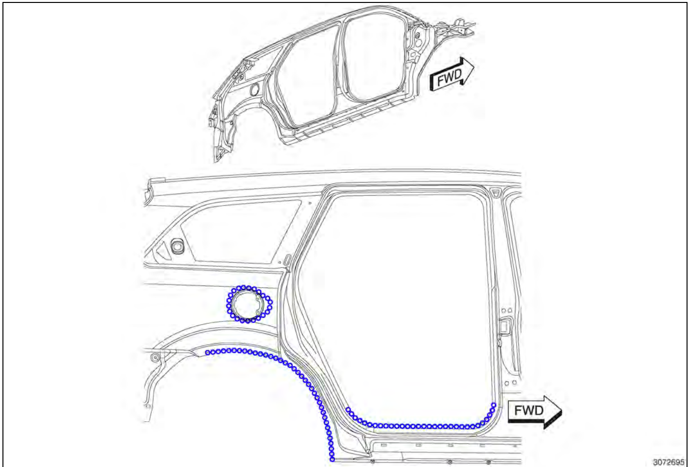
Fig. 47 Body Side Aperture/Rear Door Opening
