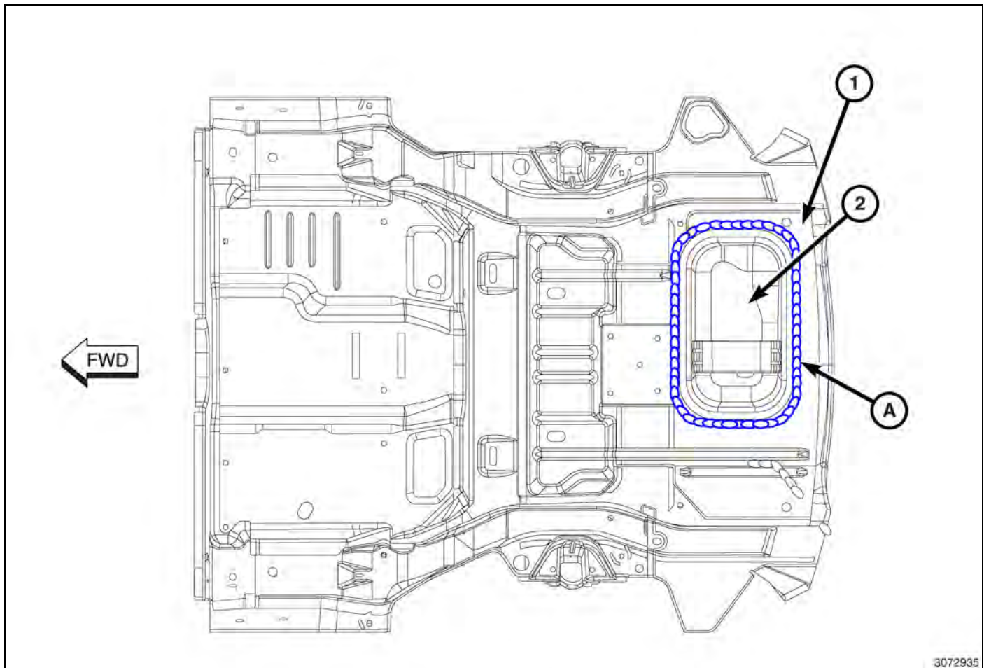
Fig. 49 Rear Floor Storage Bin
