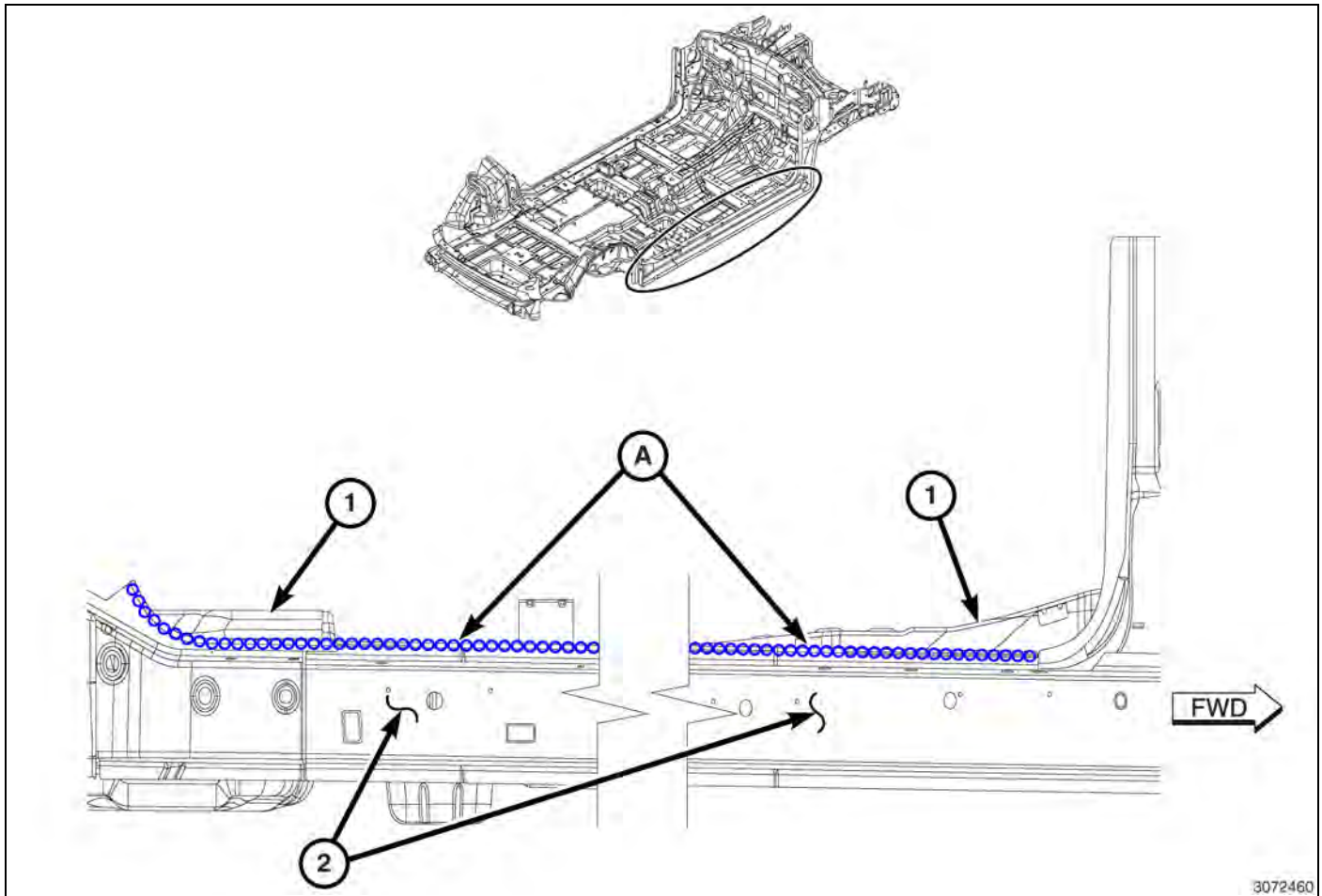
Fig. 36 Side Sill to Floor Pan
