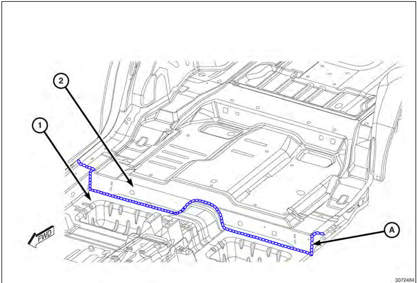
Fig. 38 Front Floor Pans TO Crossmember
