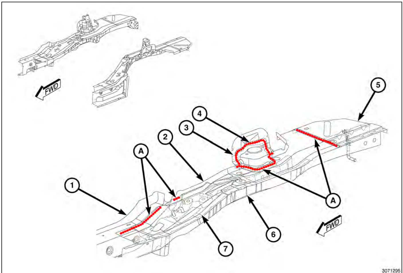
Fig. 65 Side Member (2 of 2)
