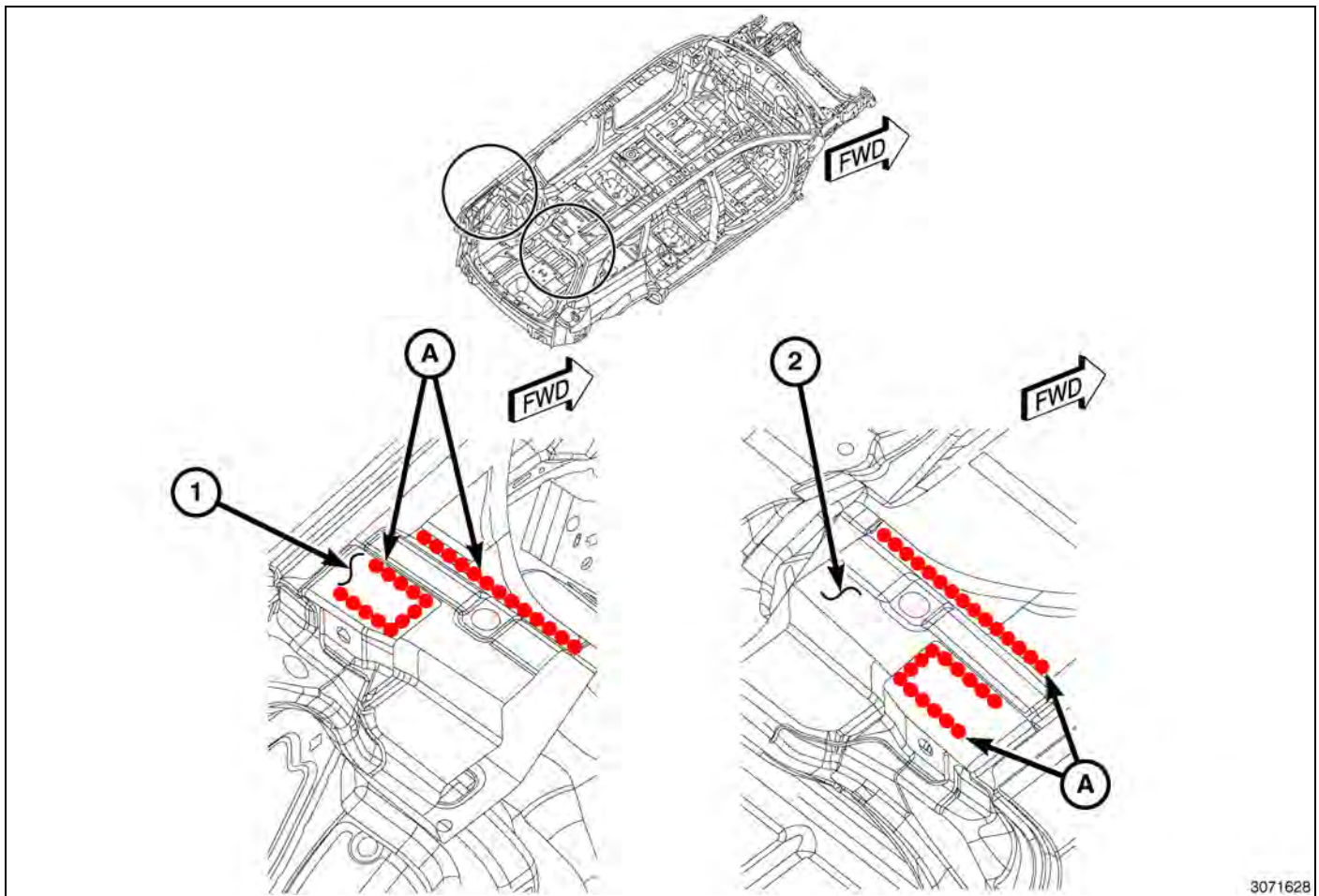
Fig. 78 Body Side Aperture/ Rear Header
