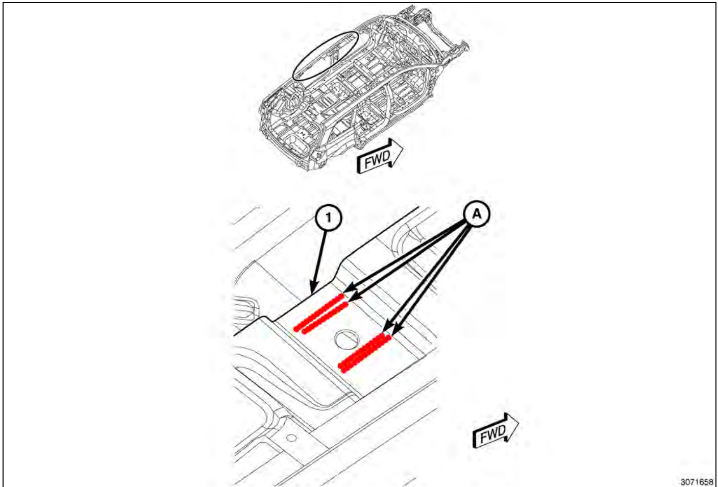
Fig. 79 Body Side Aperture/Roof Bow (Typical)
