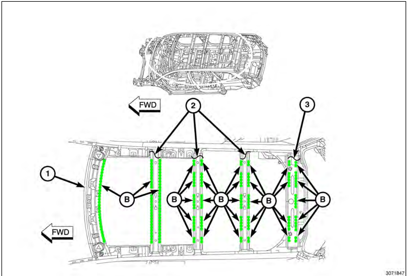
Fig. 81 Roof Bows/Roof Panel
