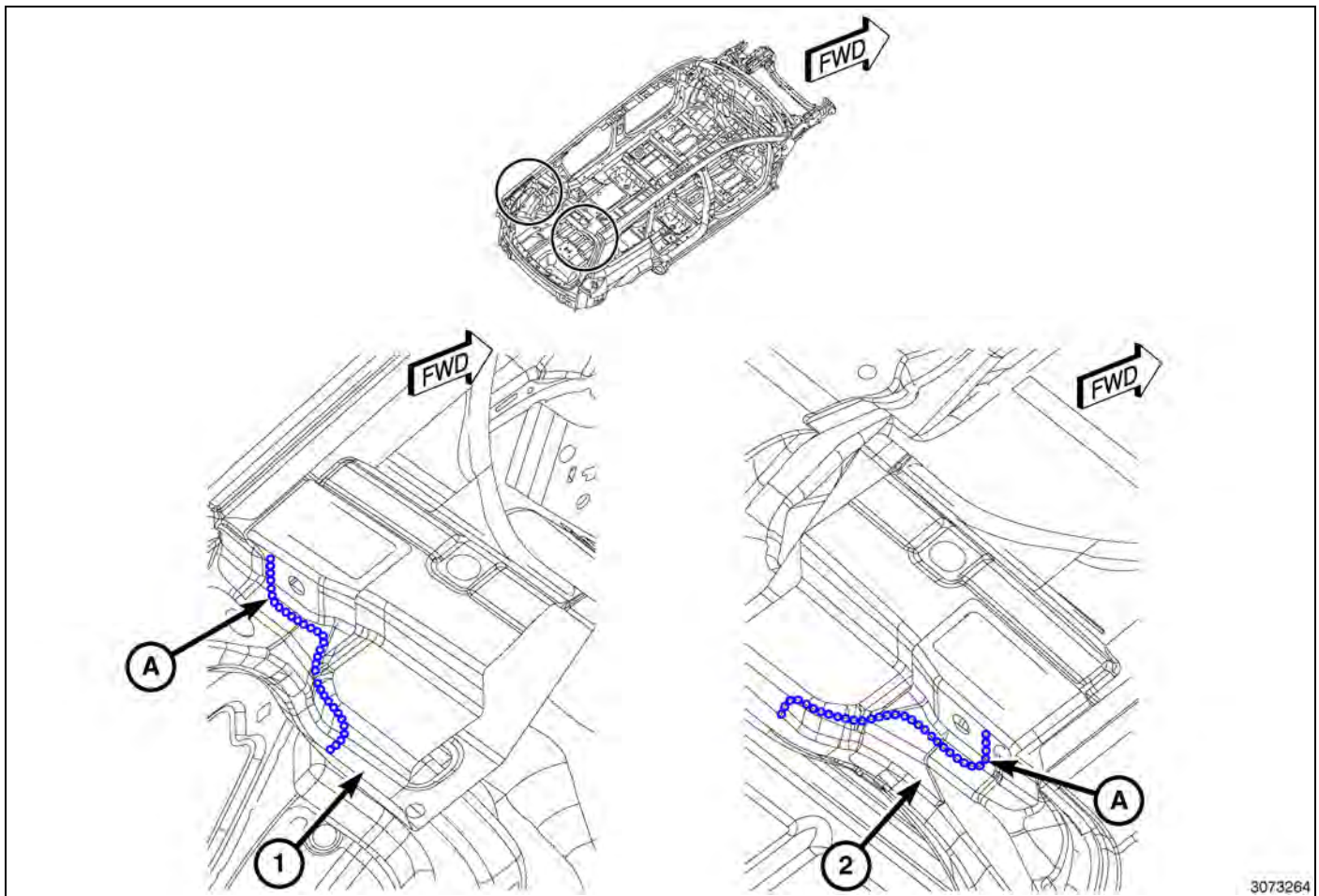
Fig. 52 Liftgate Opening
