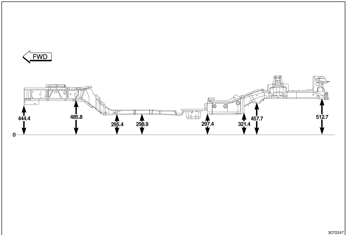
Fig. 8 Underbody Side View
