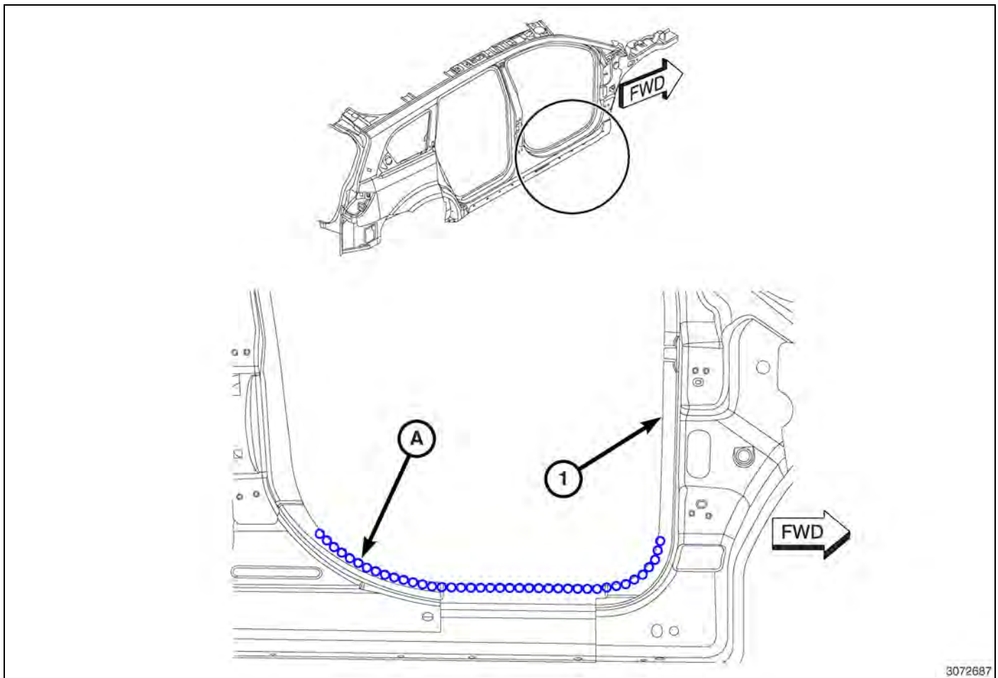
Fig. 46 Body Side Aperture/Lower Front Door Opening
