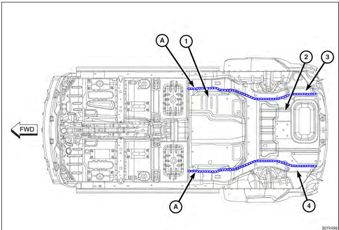
Fig. 39 Mid Floor Pan/Rear Floor Pan To Sidemember
