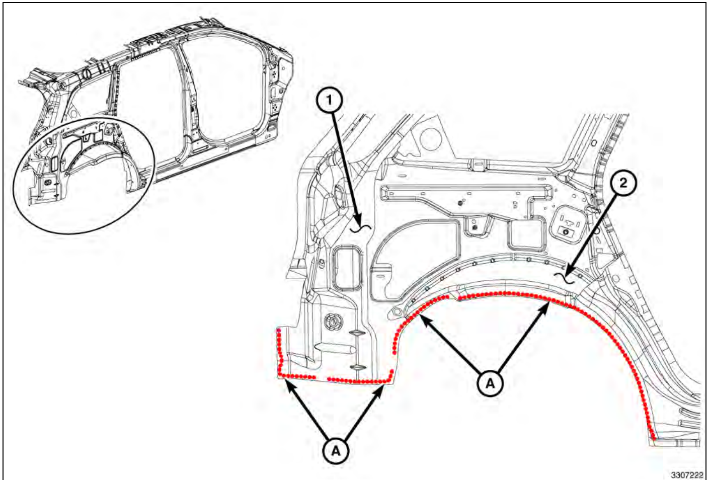
Fig. 71 Right Outer Wheelhouse
